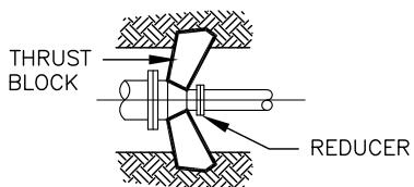
REDUCER PLAN VIEW
