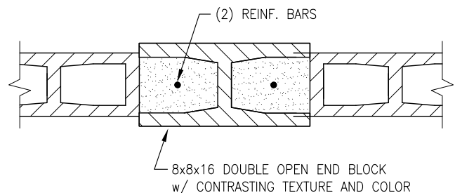
4 PILASTER DETAIL
