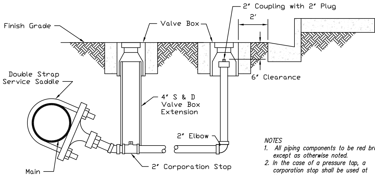
TYPICAL FLUSHOUT PERMANENT INSTALLATION
