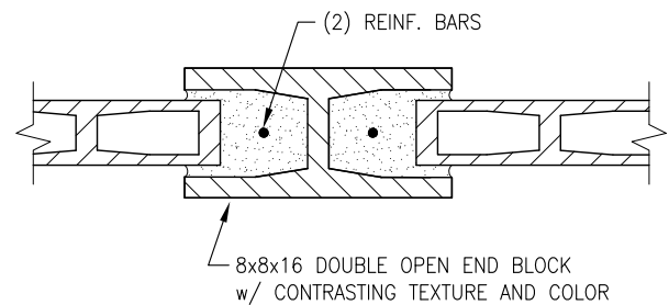
2 PILASTER DETAIL
