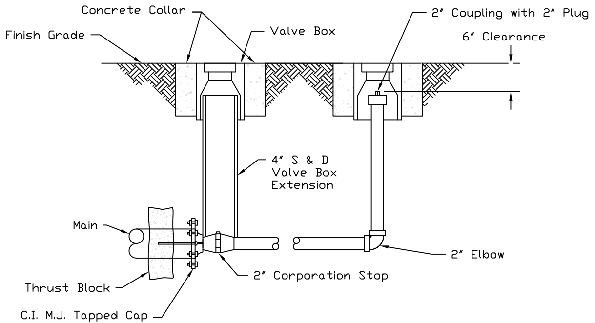
TYPICAL BLOWOFF DEAD END
